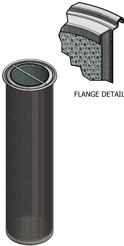
PLEATED #2 SE BASKET
