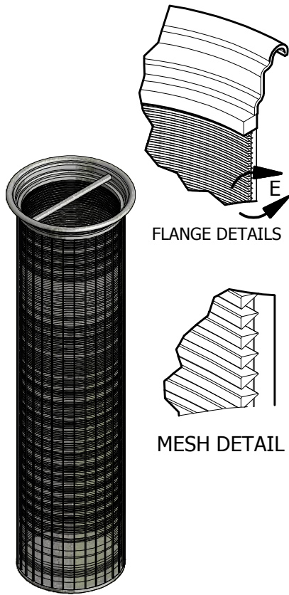
WEDGE WIRE BASKET
