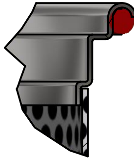
BASKET FLANGE DETAIL
