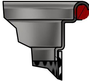
BASKET FLANGE DETAIL
