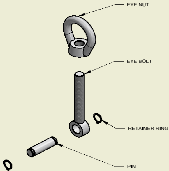
EYE BOLT STANDARD SET (FROM 1/2" TO 5/8" DIAMETER COME WITH EYE NUT)
