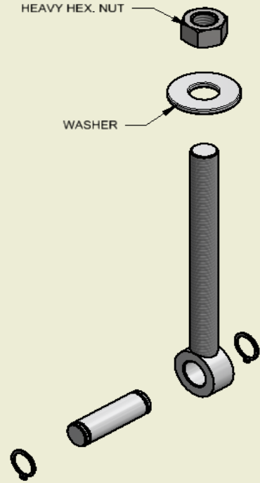
EYE BOLT STANDARD SET (FROM 3/4" DIAMETER AND UP COME WITH HEAVY HEX NUT)
